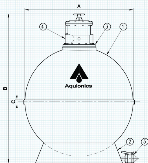
JOHOR SERIES – FRONT SCALE : N.T.S
