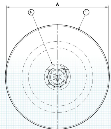
JOHOR SERIES – PLAN SCALE : N.T.S
