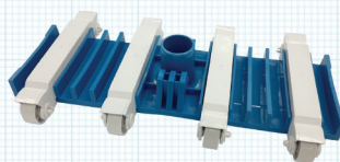
14" Flexible Vacuum Head Pleco V30 350mm wide. 40mm connection
