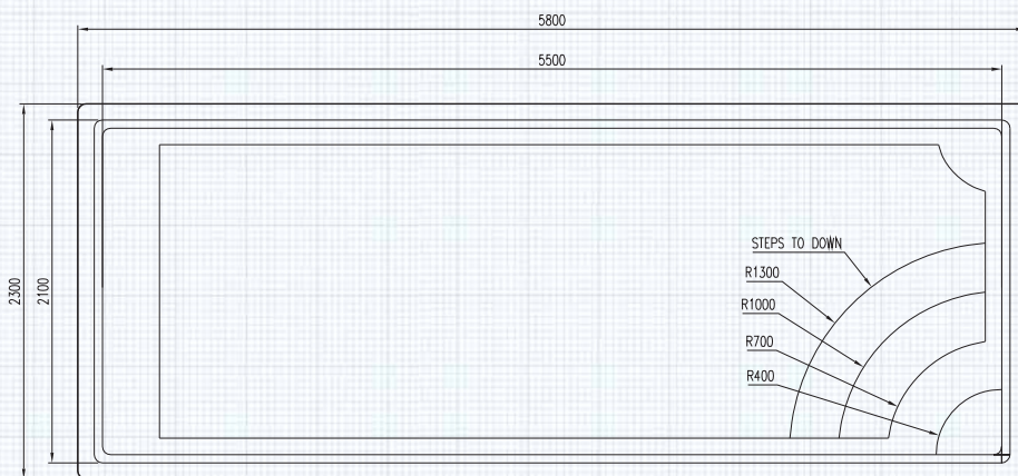
PLAN VIEW SCALE 1:25
