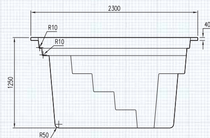
RIGHT VIEW SCALE 1:25
